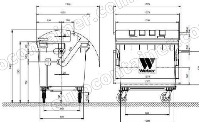
Waste Container from Weber Dimensions of the 1100 Litre Round Lid Sizes and Measures
